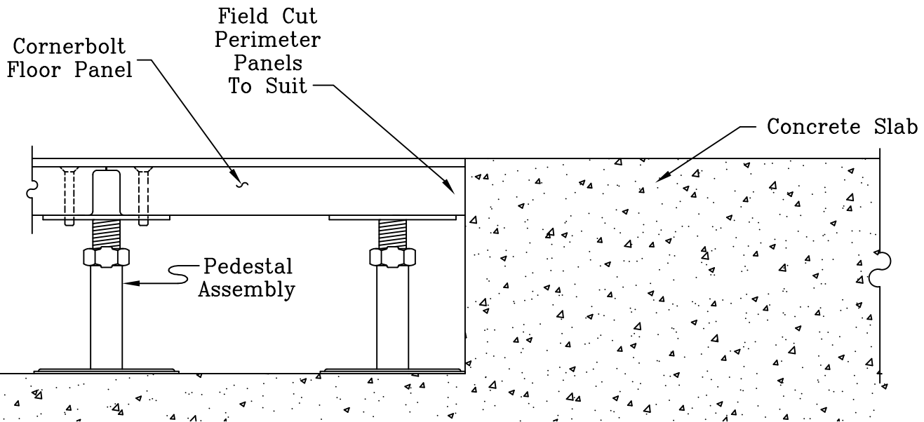
PERIMETER AT DEPRESSED SLAB
